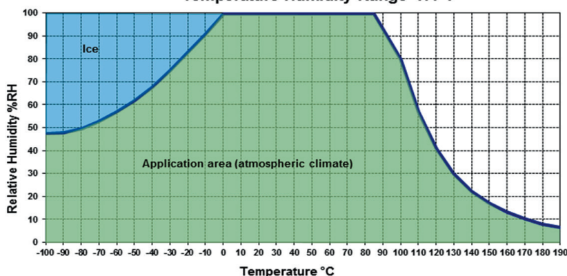
Temperature-Humidity-Range HT-1
